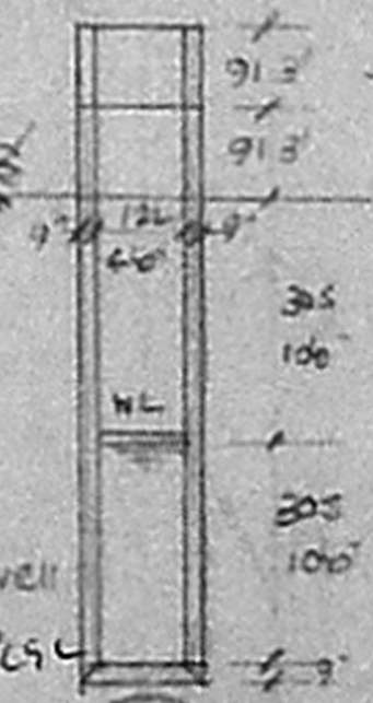
PLAN & SEC. OF SEPT. TANK
