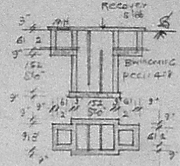
PLAN & SEC. OF SEPT. TANK
